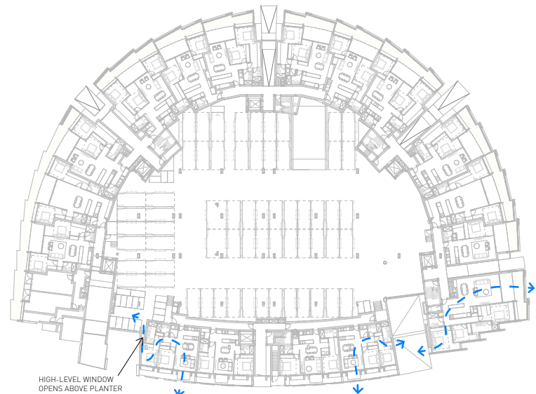
1 CROSS-VENTILATION - GROUND 1 : 500
