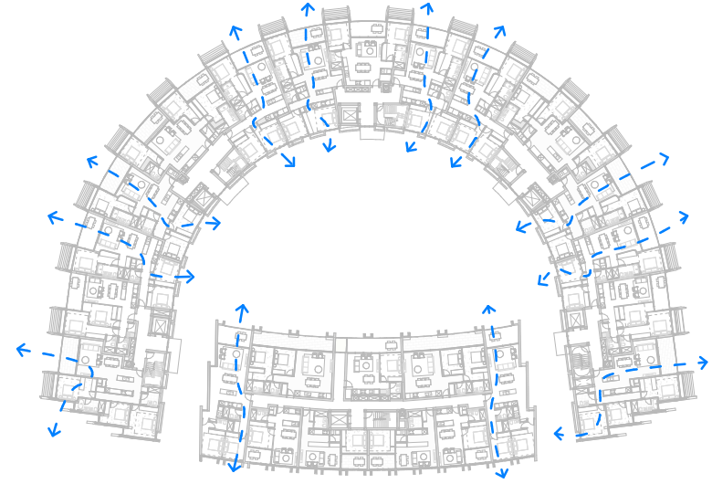
3 CROSS-VENTILATION - L02 1 : 500
